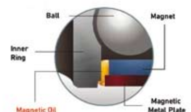
CUTAWAY DIAGRAM
